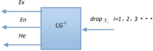
Figure 3 One-dimensional reverse cloud generator
